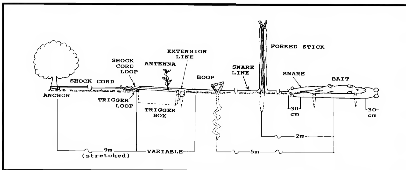
Figure 2. Application of radio-controlled trigger box to Hertog's power snare. Distance relationships between bait, snare, forked stick, and hoop are from Hertog (1987).
